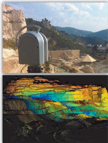
Figure 4: Quarry photo and point cloud of long range TX8 scan
